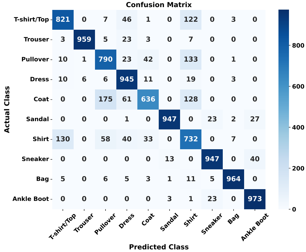
Figure 7: Confusion Matrix
