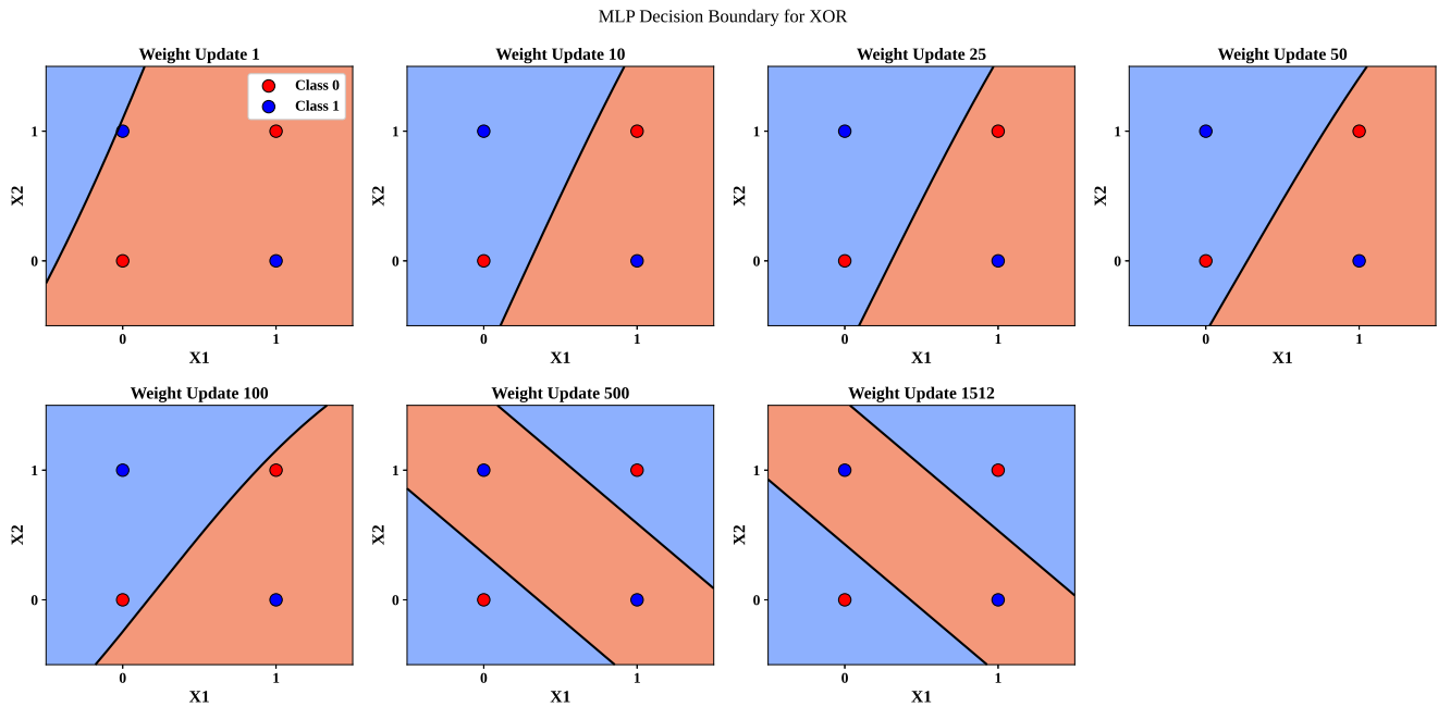
Figure 10: Decision Boundaries for XOR Gate Using MLP
